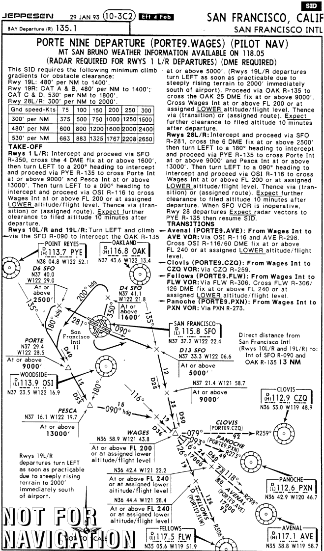
Reproduced with permission of Jeppesen Sanderson, Inc. Reduced for illustrative purposes Figure 5-43
